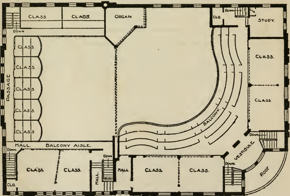
SECOND FLOOR PLAN FIRST CHRISTIAN CHURCH, ATHENS, GA.
